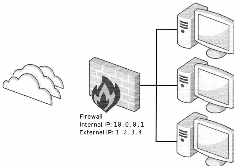
Figure 4.1: A sample network layout for NAT
