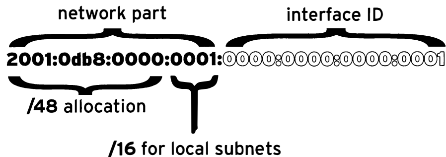
Figure 2.1: IPv6 address parts and subnetting
