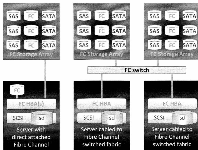
Figure 7.2: Fibre Channel block storage topologies
