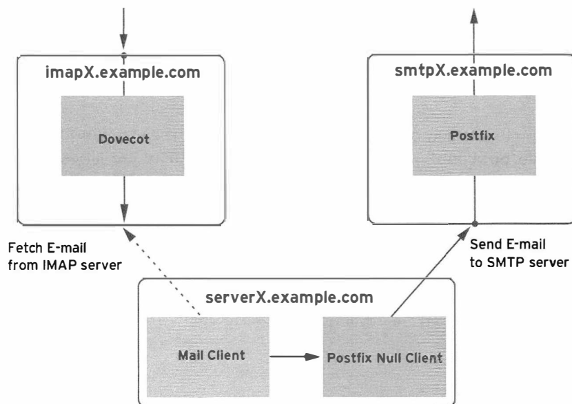
Figure 6.2: Null client communication
