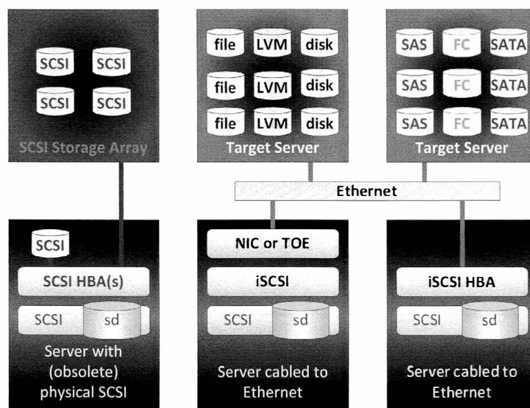
Figure 7.1: SCSI and iSCSI block storage topologies
