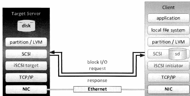
Figure 7.3: Block I/O network stack components
